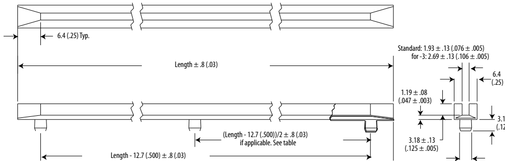
Series C120 - Nylon Guide (conductive)
